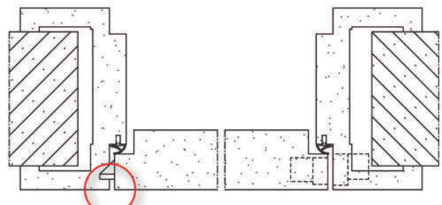
Element in Stumpfoptik, EE Zarge
